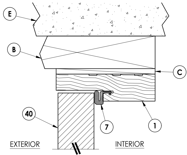
1 VERTICAL CROSS SECTION 5 Outswing shown (Inswing similar)
