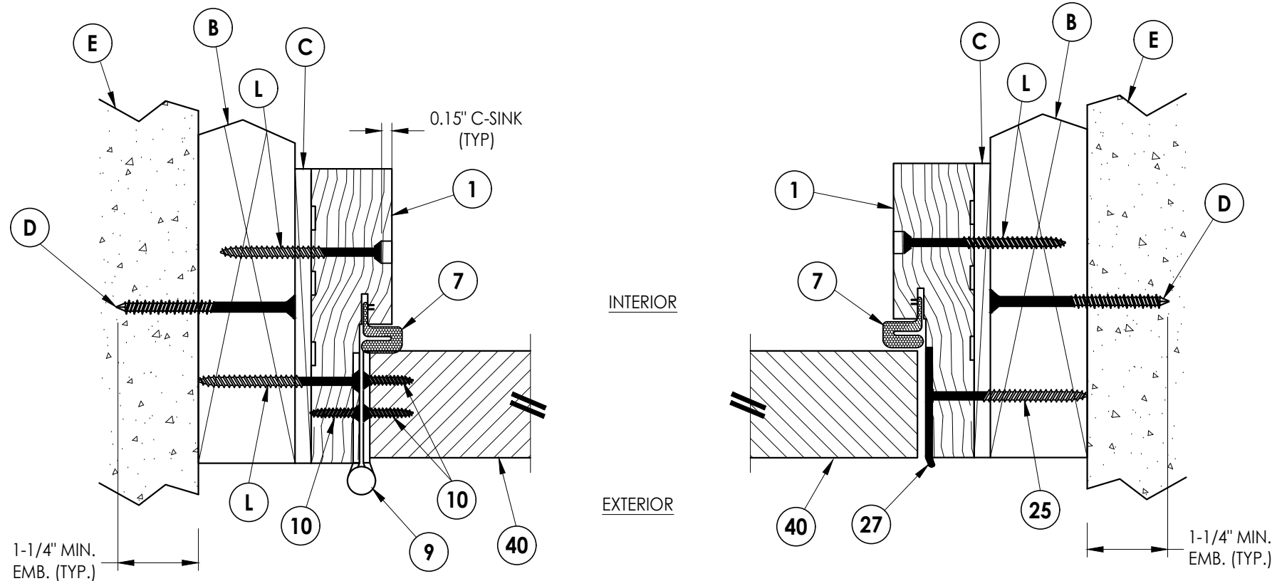
2 HORIZONTAL CROSS SECTION 5 Outswing shown (Inswing similar)
