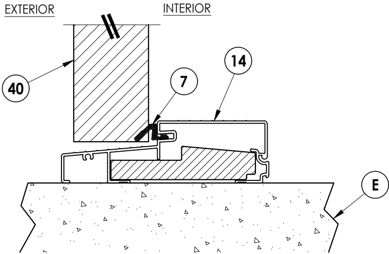
2 8 VERTICAL CROSS SECTION Outswing Threshold
