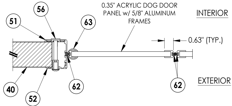
2/4 HORIZONTAL CROSS SECTION
